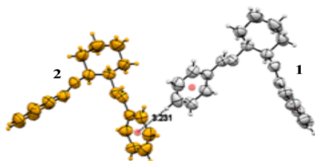
Figure 3: C-H...π (arene) interaction between 1 and 2.
